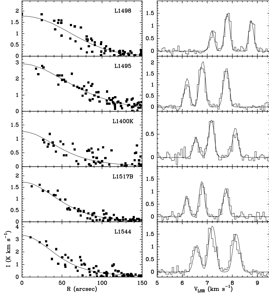
FIG. 5.— Radial profiles of integrated emission (left) and central emerging spectrum (right) for \text{N}_2\text{H}^+(1-0) . Observations are indicated by solid squares in the radial profiles (sum of all hyperfine components) and by histograms in the spectra (all temperature units are in the main beam scale). Constant abundance models are indicated by solid lines, and unlike the case of \text{C}^{18}\text{O} and CS (Fig. 3), they accurately fit the data at all radii (see parameters in Table 4). For the emerging spectra, only the central hyperfine group is presented to show in detail the good matching of both the linewidth and the hyperfine ratios. To use the same velocity scale in all the spectra, both data and model for L1400K have been shifted by 4 \text{ km s}^{-1} , and by 1 \text{ km s}^{-1} for L1517B.
